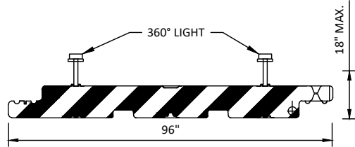
A LOW PROFILE BARRICADE DETAIL G2.02 NOT TO SCALE
