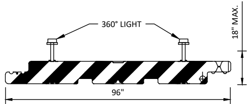
A G2.01 LOW PROFILE BARRICADE DETAIL NOT TO SCALE
