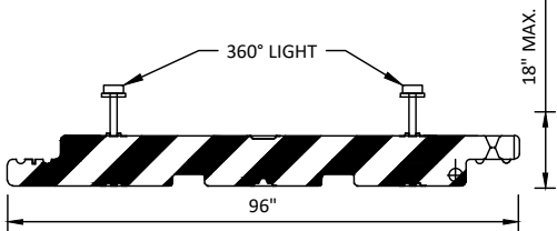
A G2.03 LOW PROFILE BARRICADE DETAIL NOT TO SCALE
