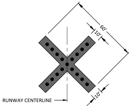
B LIGHTED RUNWAY CLOSURE MARKER G2.02 NOT TO SCALE
