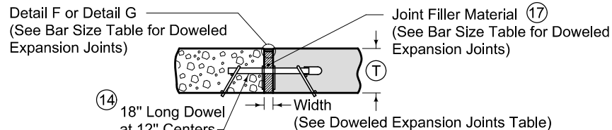
'ED', 'EE', 'EF' (16) DOWELED EXPANSION JOINT
