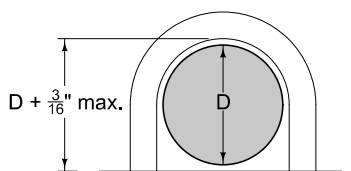
BEND AROUND DOWEL ③1
