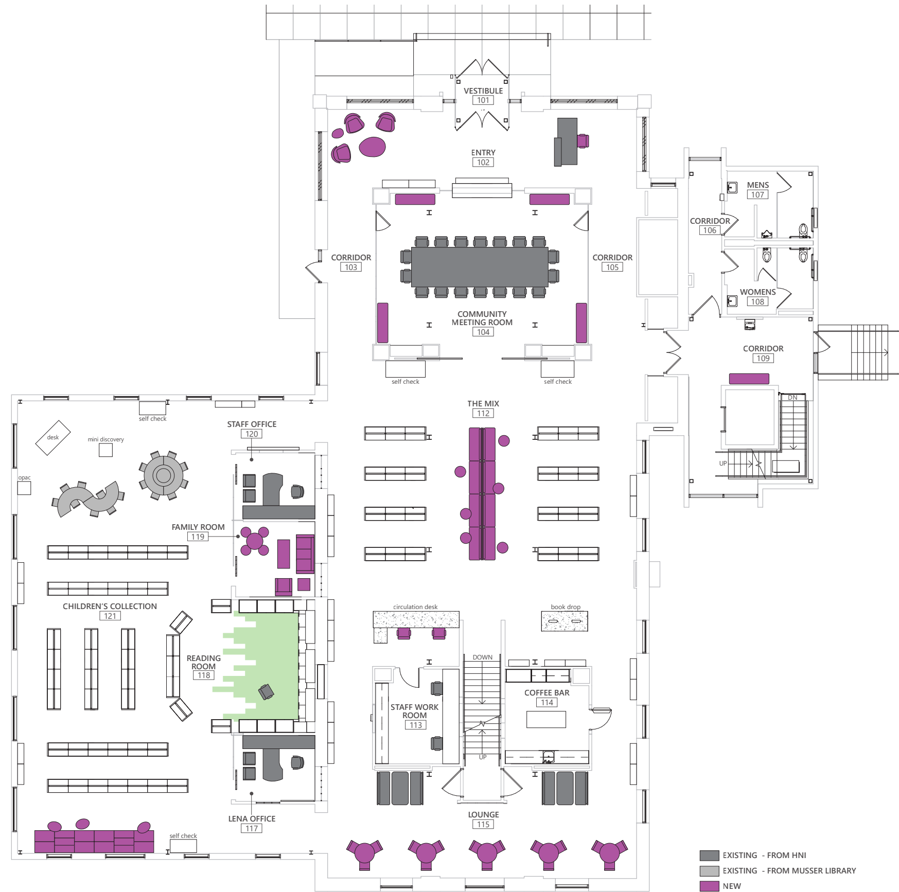
1 FURNITURE FLOOR PLAN LEVEL 1 Scale: Not to Scale
