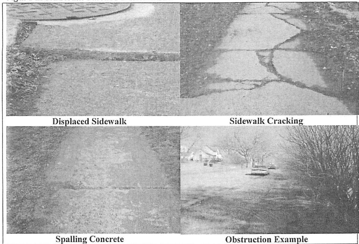
Figure 1: Sidewalk Surface Deficiencies 5
