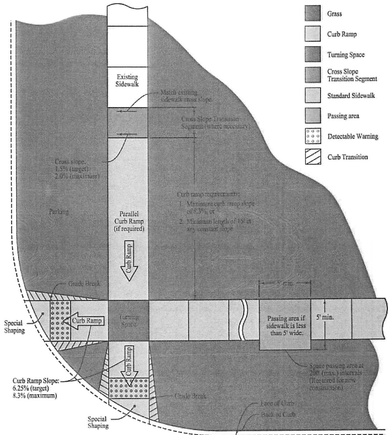
Figure 2: Standard Sidewalk and Curb Ramp Elements
