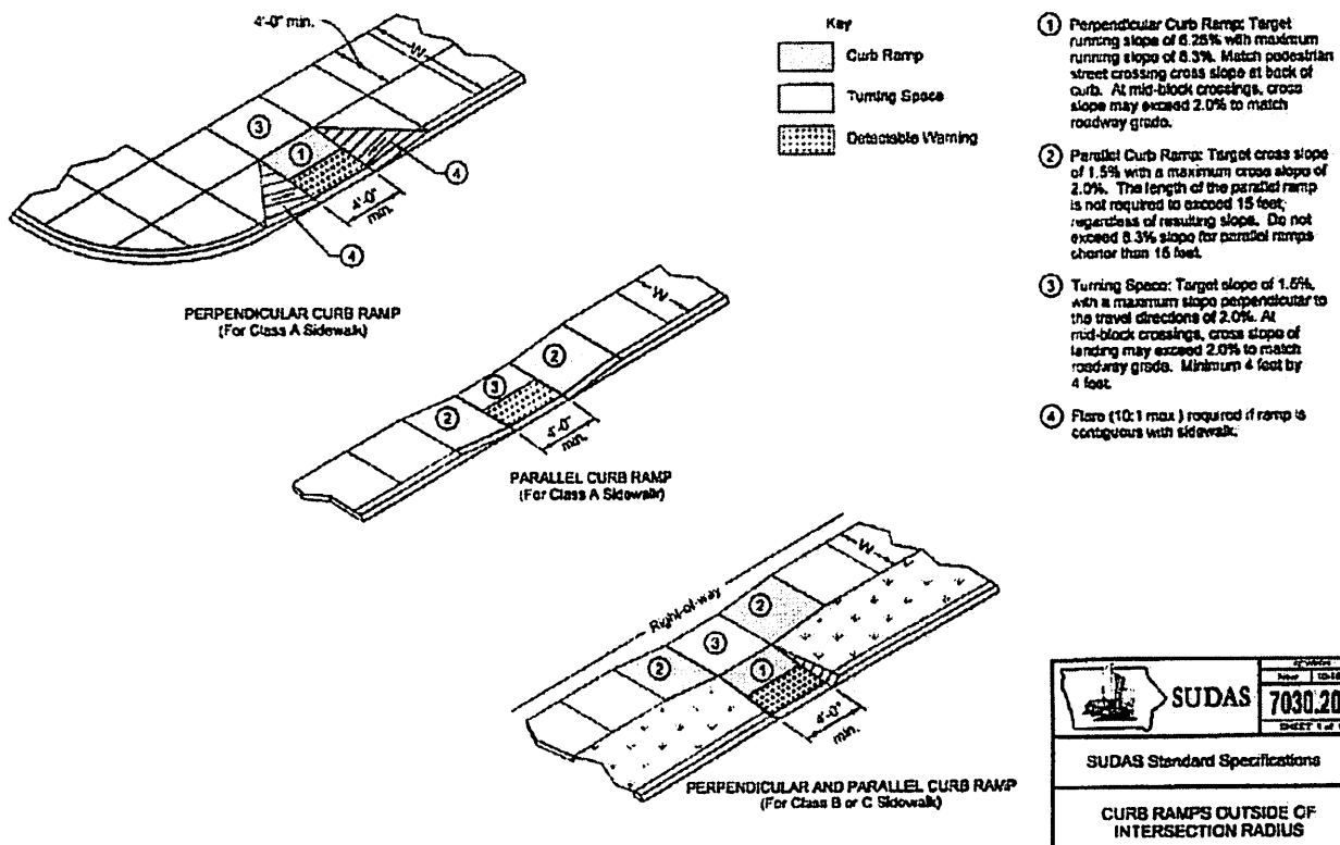
Figure 4: Curb Ramps Outside of Intersection Radius
